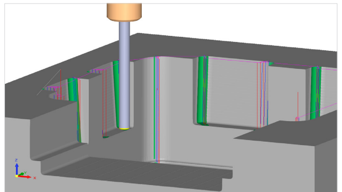
An efficient re-rouging at corners is done with the new "Corner Plunging" procedure, where the stock is removed by down cutting operations, including an option for forward steps.
